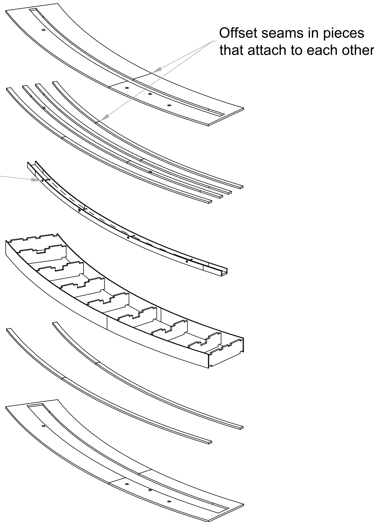
7 SEPARATED ISO VIEW Scale: NTS
