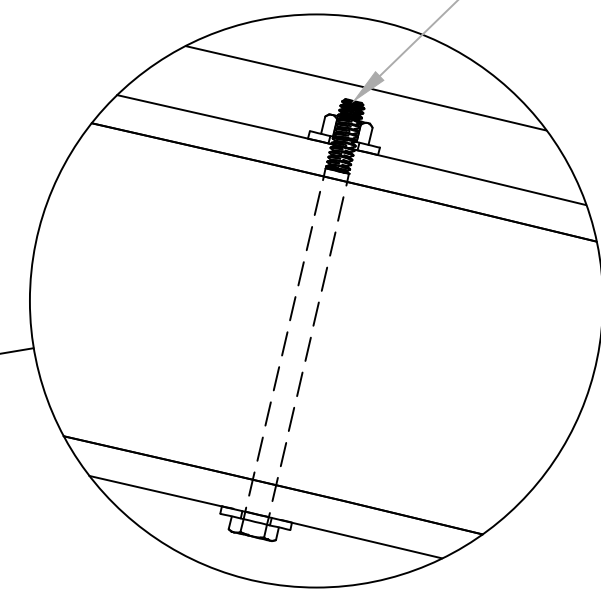
DETAIL C SCALE 6" = 1'-0"
