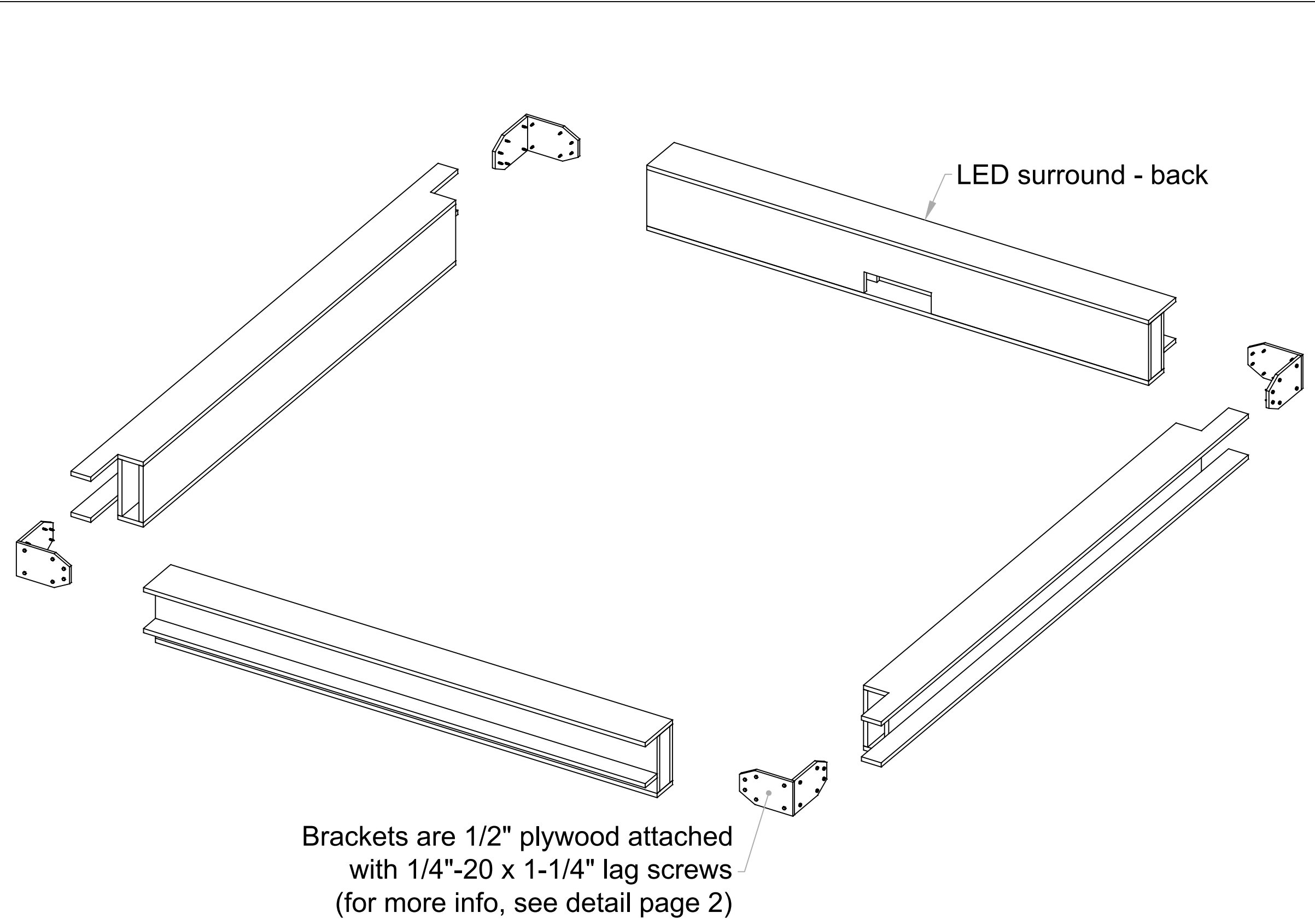
5 SEPARATED ISO VIEW Scale: NTS
