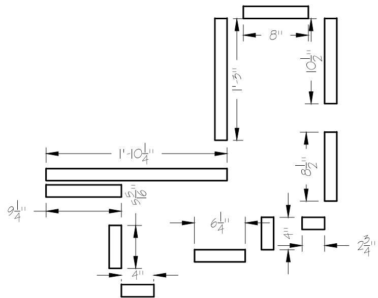
1 200 COLUMN INTERNAL MEMBERS - TOP VIEW 1 = 1'-0'' USE 2X4 CUT FIVE OF EACH FOR ONE COLUMN (TEN OF EACH TOTAL)
