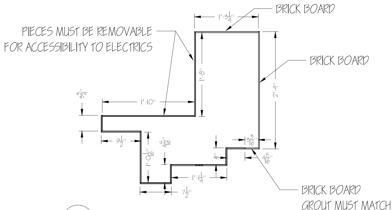
3 200 COLUMN FACING - TOP VIEW 1 = 1'-0'' UNLESS SPECIFIED, ALL FACING IS 1/4" Luan CUT ONE OF EACH FOR ONE COLUMN (TWO OF EACH TOTAL) PAY ATTENTION TO WHICH BOARDS CAP WHICH ENDS
