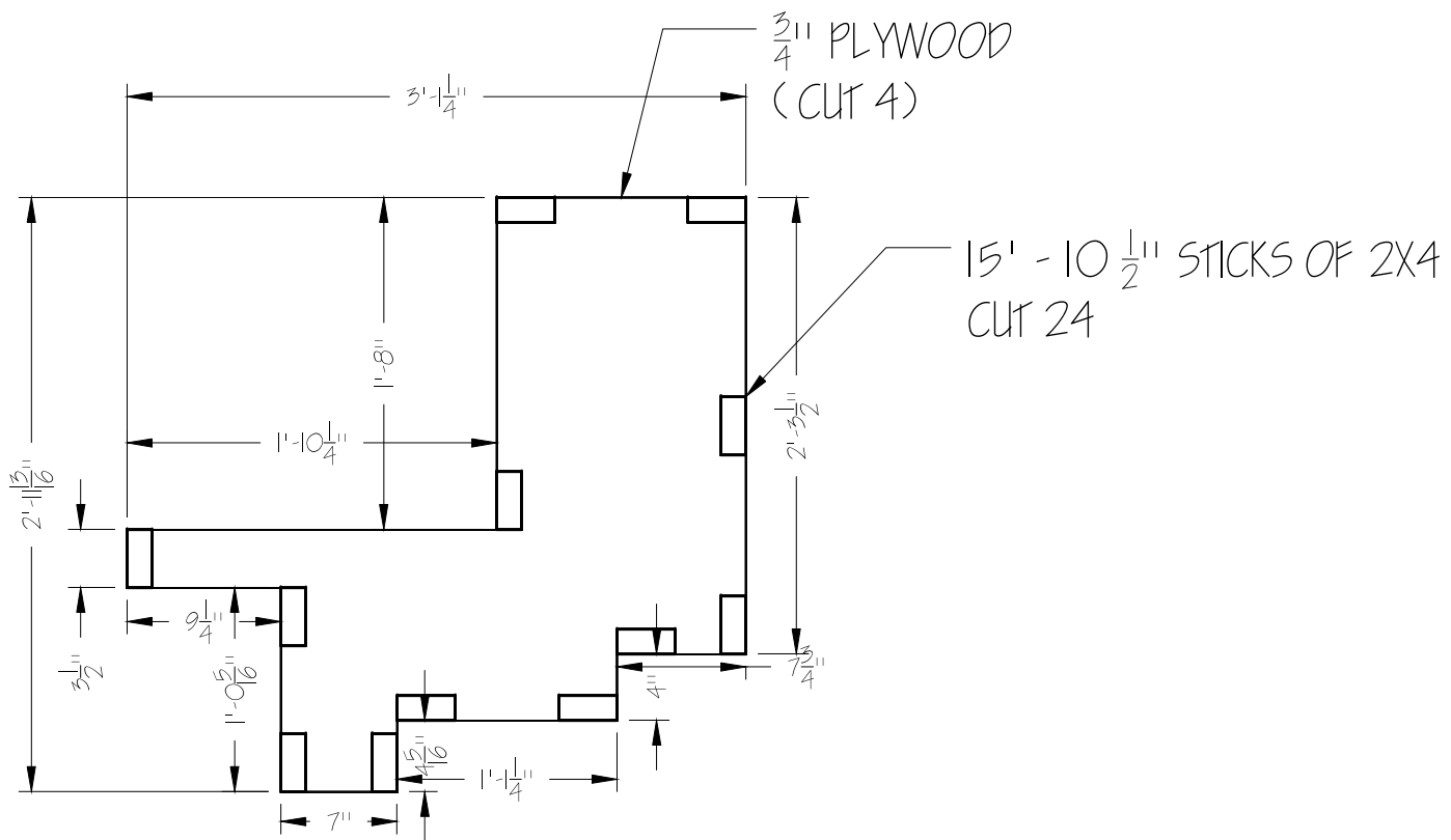
2 200 COLUMN LIDS AND VERTICALS - TOP VIEW 1 = 1'-0'' CUT TWO (ONE IS R&R)
