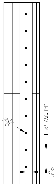
3 200 COLUMN FACING - FRONT VIEW 1/4'' = 1'-0'' INCLUDES LAYOUT OF HOLES FOR LAMP SOCKETS. DO NOT ATTACH REAR FACING UNTIL ELECTRICS WIRES SOCKETS.
